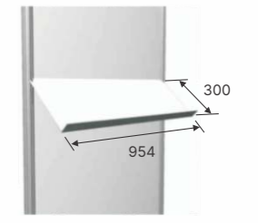
Nuožulni lentyna bukletams Inclined shelf for booklets
