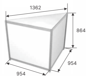
Pakyla (trikampė) Triangular platform
